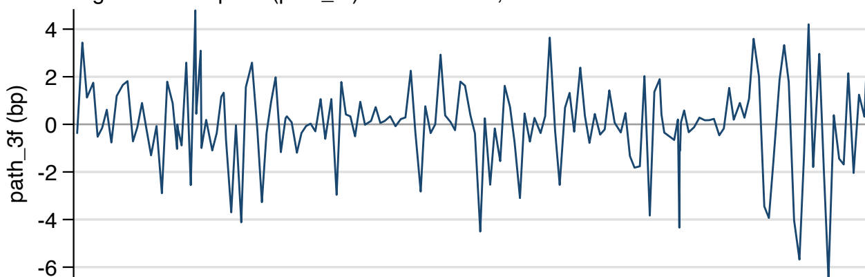
Forward-guidance surprise (path_3f) -- mean -0.00, SD 1.81
