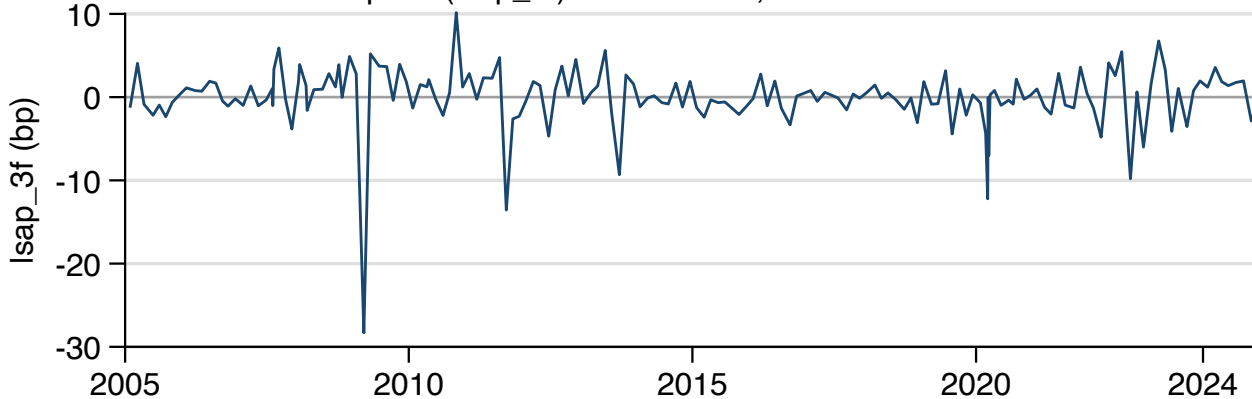
LSAP / balance-sheet surprise (lsap_3f) -- mean 0.01, SD 3.69
