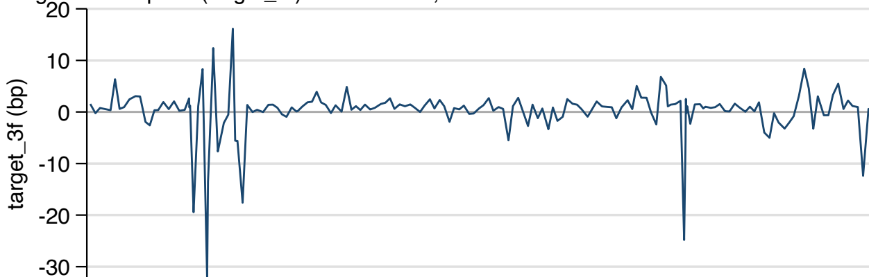
Target rate surprise (target_3f) -- mean 0.20, SD 4.89
